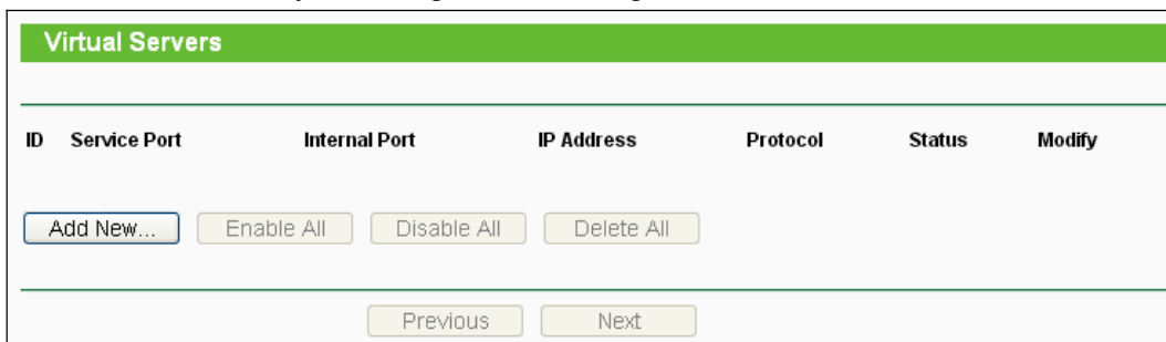
Figure 4-43 Virtual Servers
