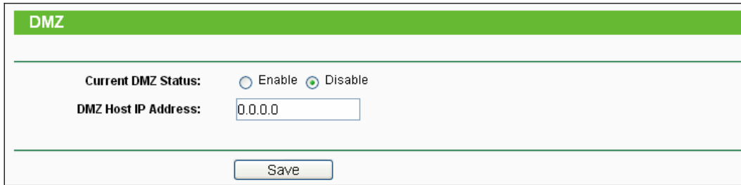
Figure 4-47 DMZ
