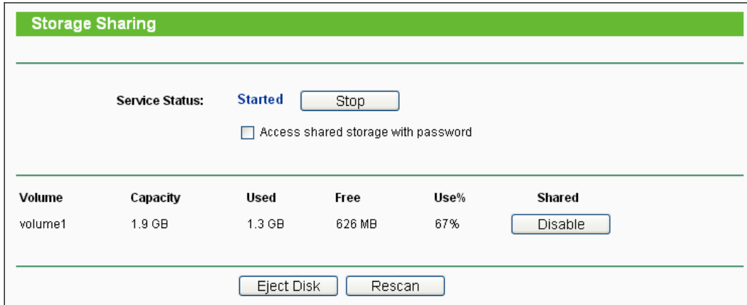
Figure 5-25 Storage Sharing
