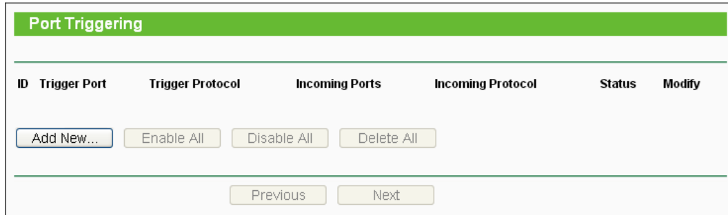
Figure 8-41 Port Triggering
