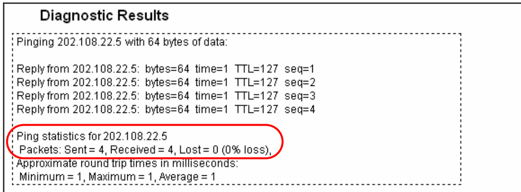
Figure 5-35 Diagnostic Results
