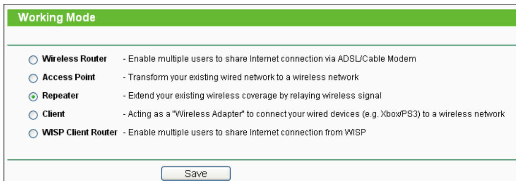
Figure 6-3 Working Mode
