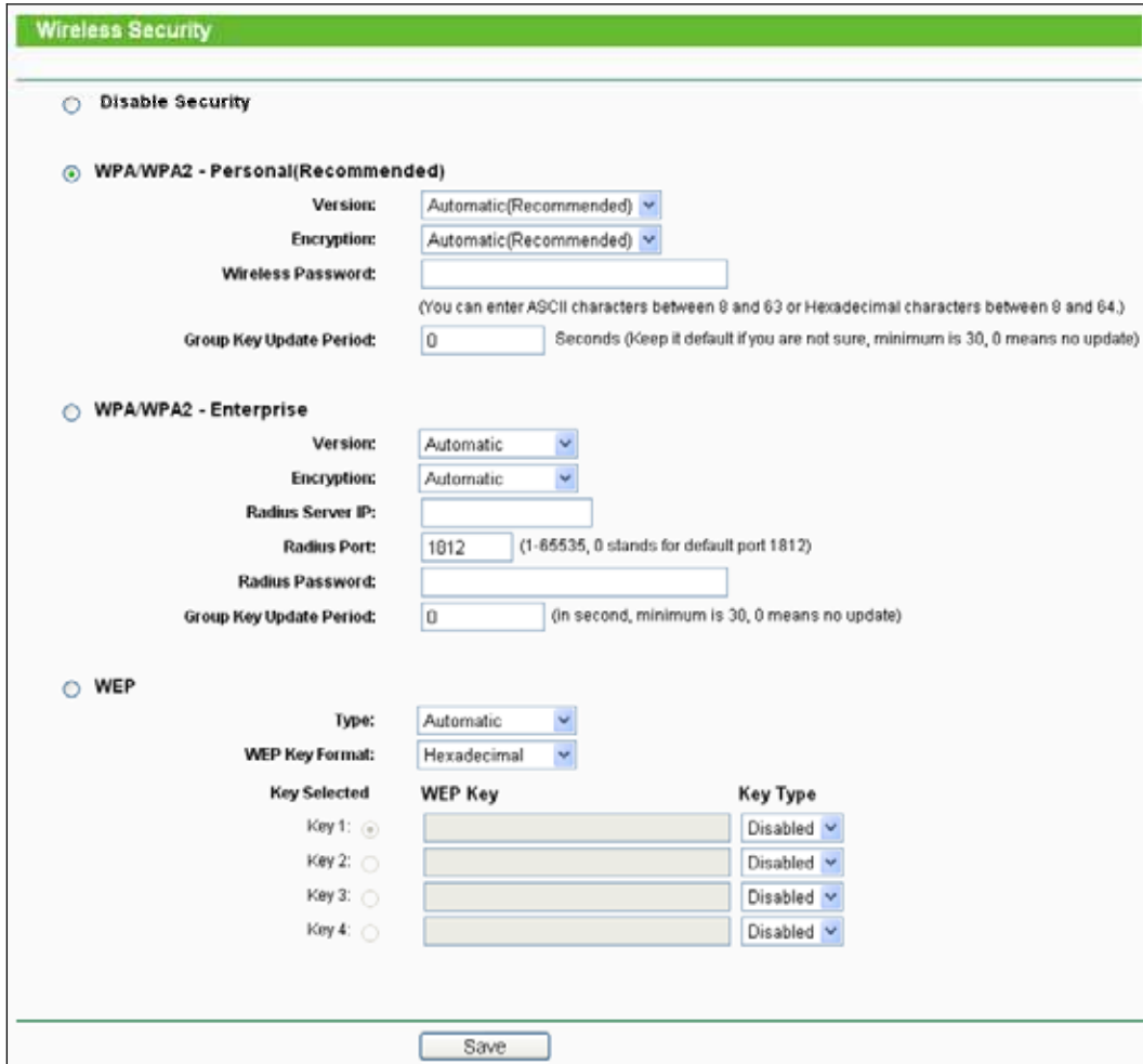
Figure 6-9 Wireless Security
