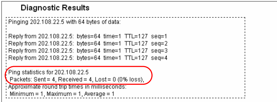
Figure 4-91 Diagnostic Results
