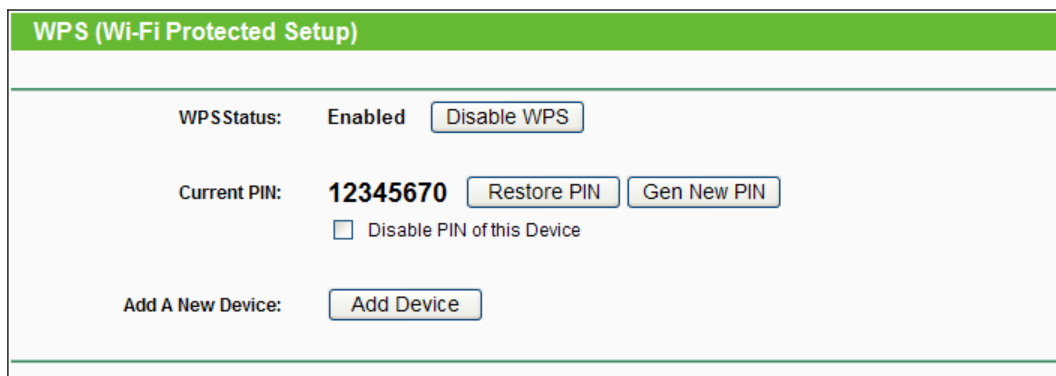
Figure 5-3 WPS
