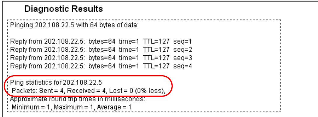
Figure 7-27 Diagnostic Results
