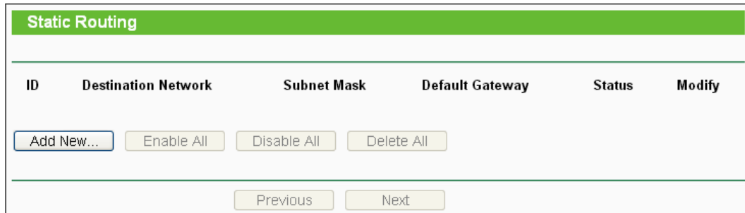
Figure 4-73 Static Routing
