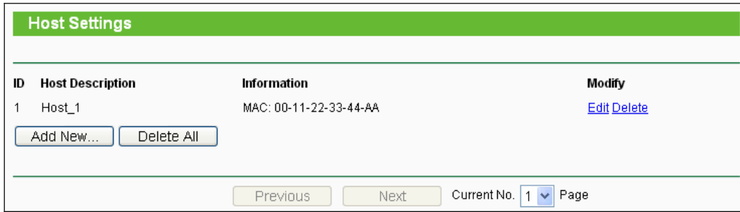
Figure 8-60 Host Settings
