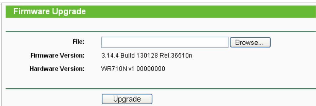
Figure 4-92 Firmware Upgrade
