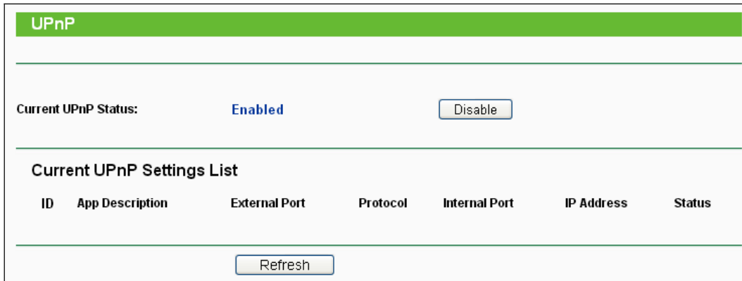
Figure 8-44 UPnP
