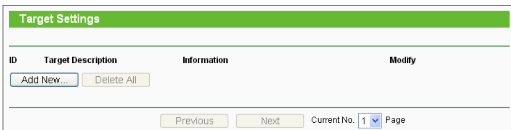
Figure 4-65 Target Settings
