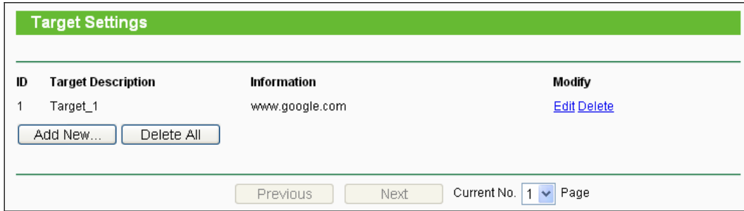
Figure 8-64 Target Settings
