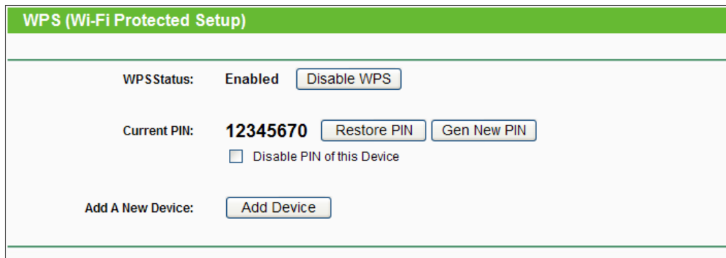
Figure 4-3 WPS
