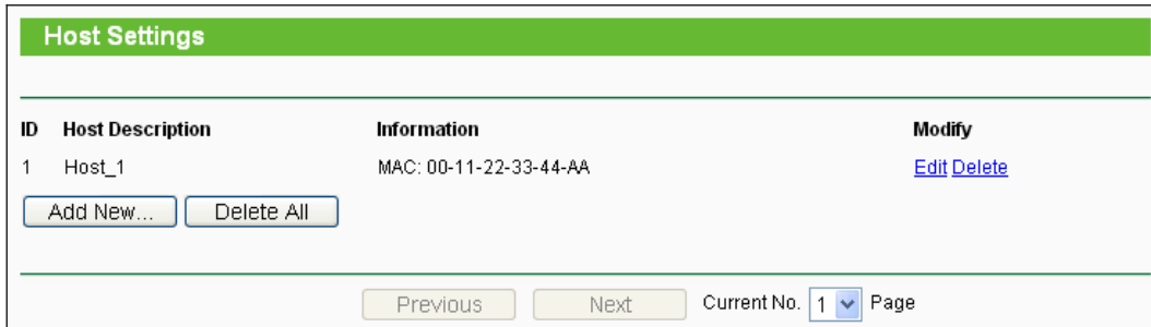
Figure 4-64 Host Settings
