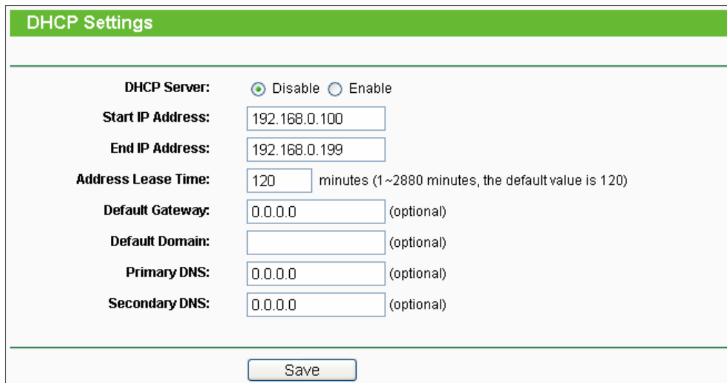
Figure 5-19 DHCP Settings
