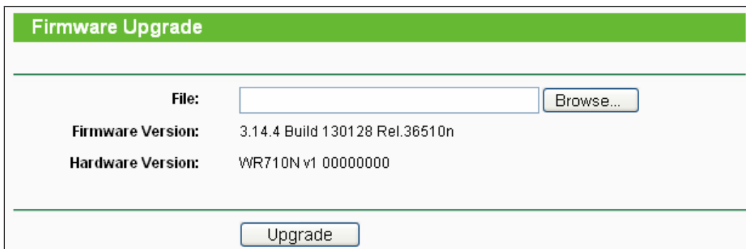
Figure 8-88 Firmware Upgrade
