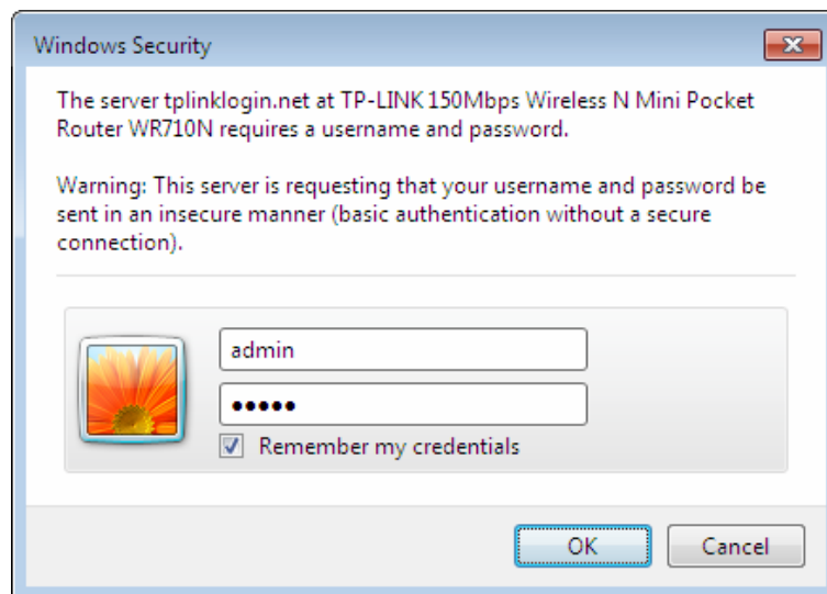
Figure 3-3 Login Windows
