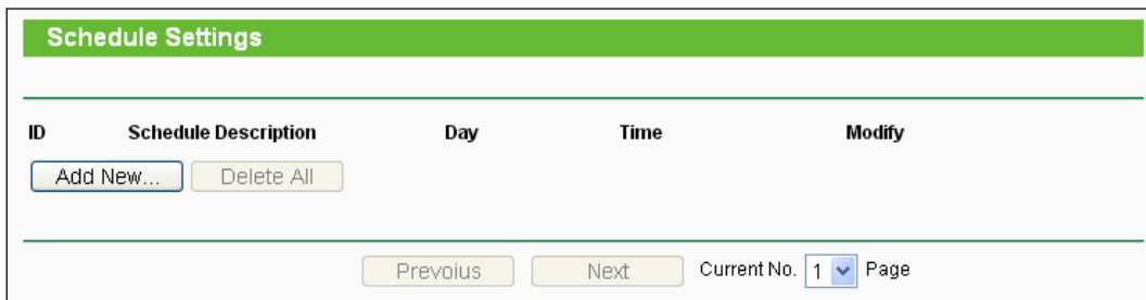
Figure 4-69 Schedule Settings
