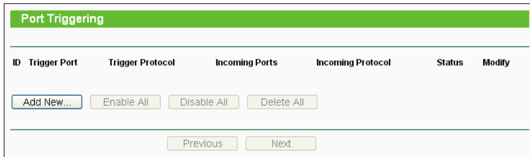
Figure 4-45 Port Triggering
