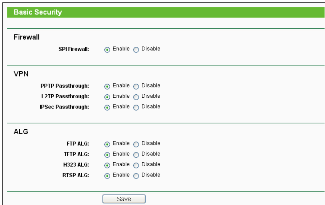
Figure 8-46 Basic Security
