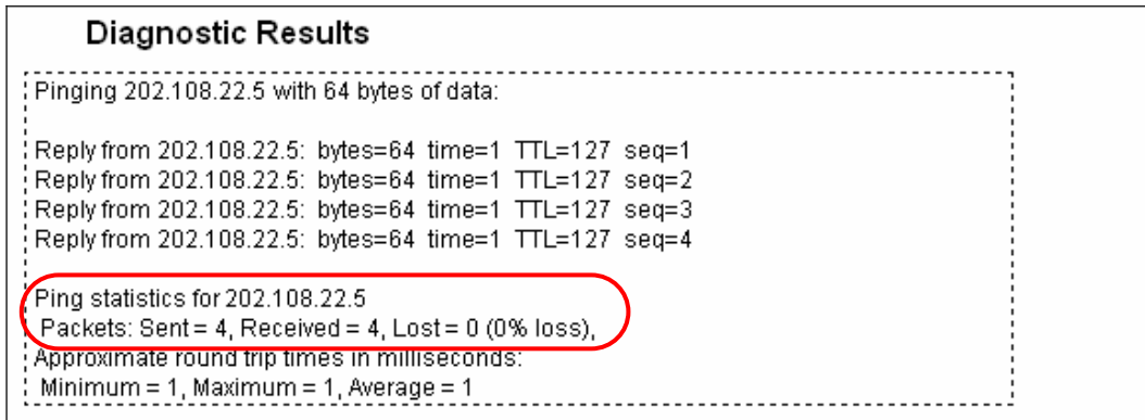
Figure 8-87 Diagnostic Results
