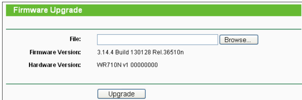
Figure 7-28 Firmware Upgrade
