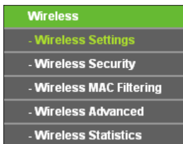
Figure 5-10 Wireless menu
