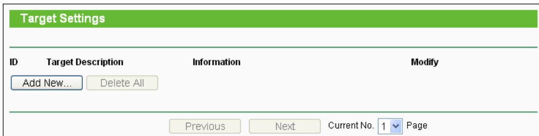
Figure 8-61 Target Settings
