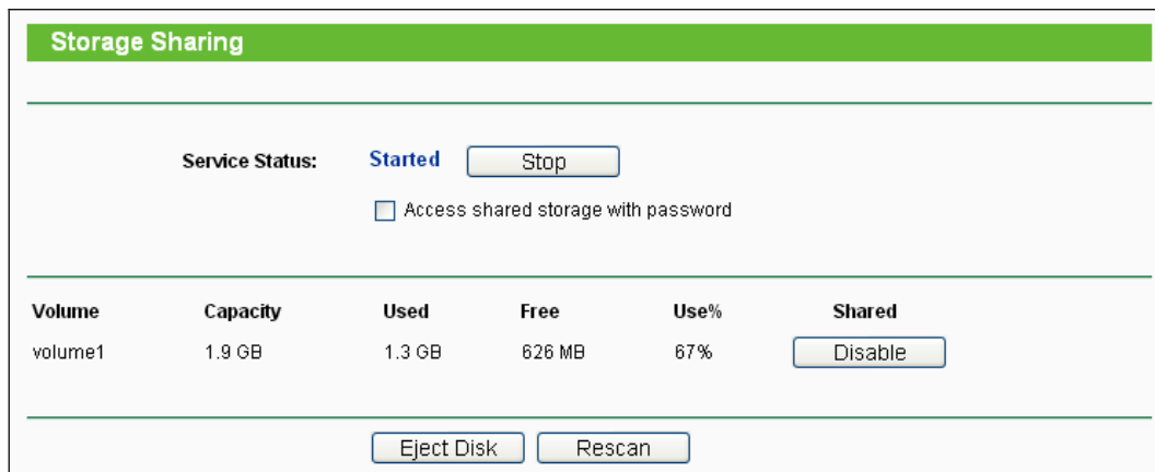
Figure 8-30 Storage Sharing
