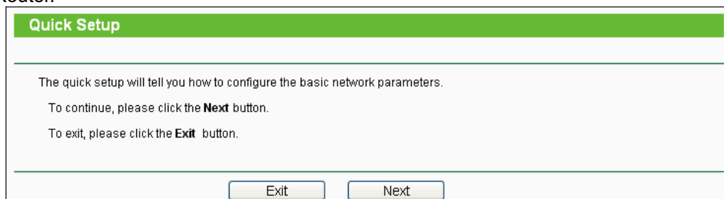
Figure 3-4 Quick Setup
