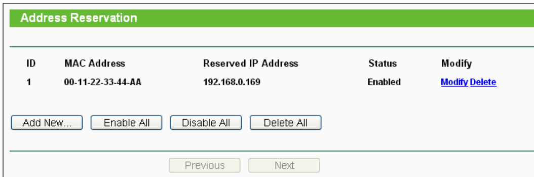
Figure 8-27 Address Reservation
