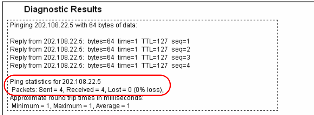
Figure 6-32 Diagnostic Results
