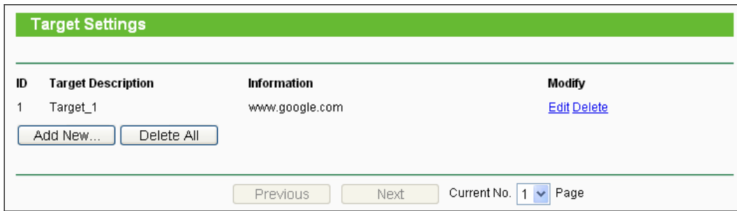
Figure 4-68 Target Settings
