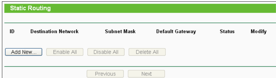
Figure 8-69 Static Routing
