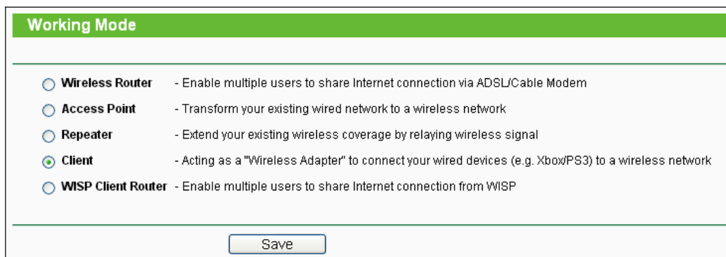
Figure 7-3 Working Mode
