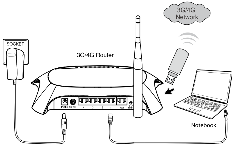
Figure 2-1 Hardware Installation of the 3G/4G Wireless N Router – 3G/4G connection
