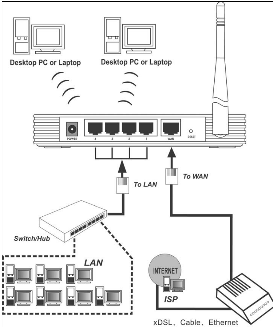
Figure 3-1 Hardware Installation of the TL-WR543G 54M Wireless AP Client Router
