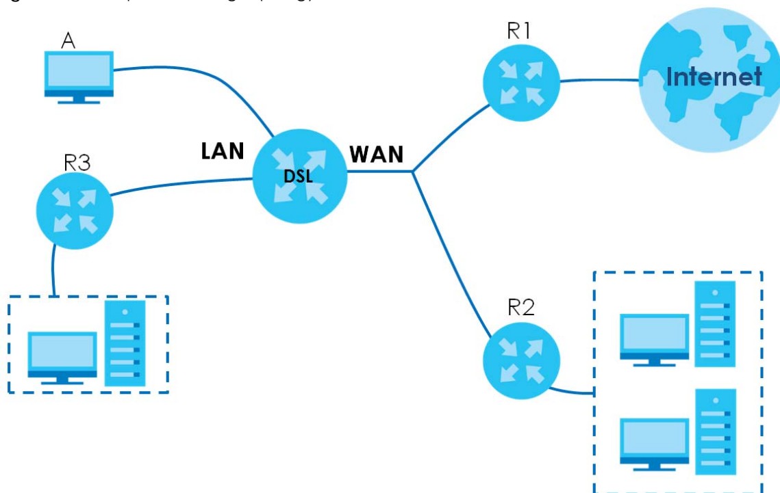
Figure 60 Example of Routing Topology
