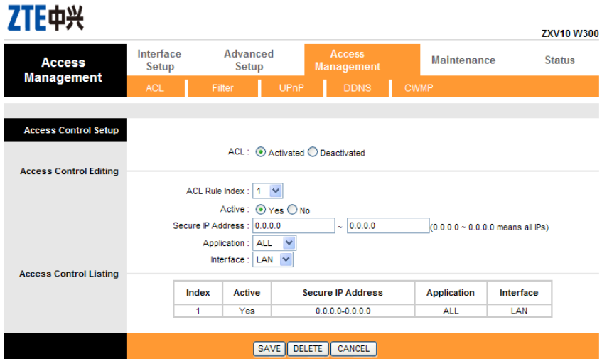
FIGURE 25 THE ACL MANAGEMENT PAGE
