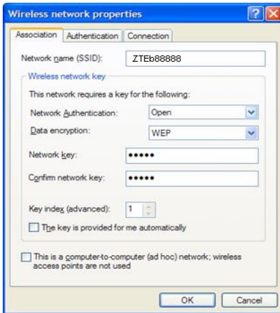
FIGURE 40 ASSOCIATION TAB (WIRELESS NETWORK PROPERTIES)
