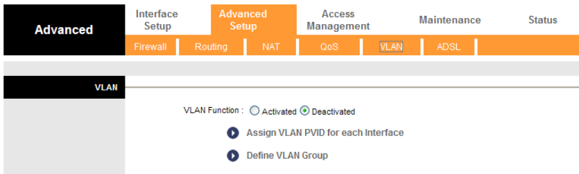
FIGURE 21 THE VLAN CONFIGURATION PAGE
