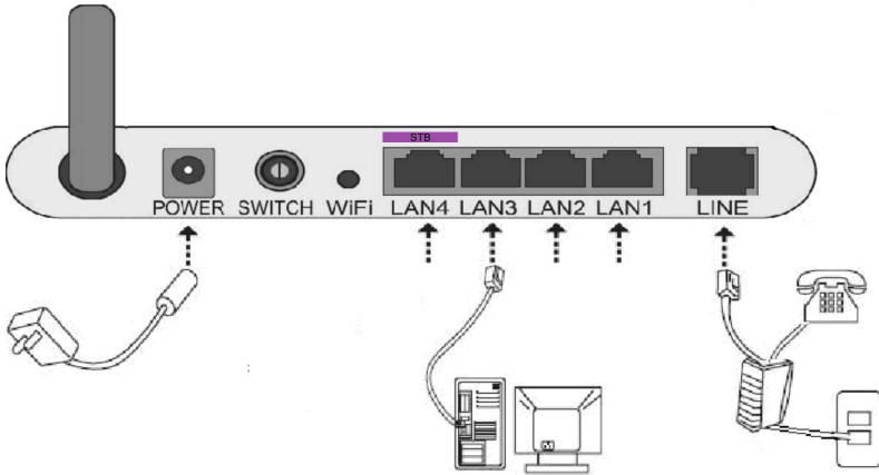
FIGURE 3 ADSL UPLINK CONNECTIONS
