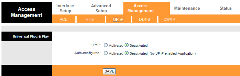
FIGURE 27 THE UPnP MANAGEMENT PAGE
