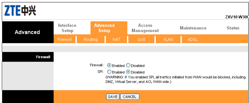
FIGURE 16 THE FIREWALL CONFIGURATION PAGE
