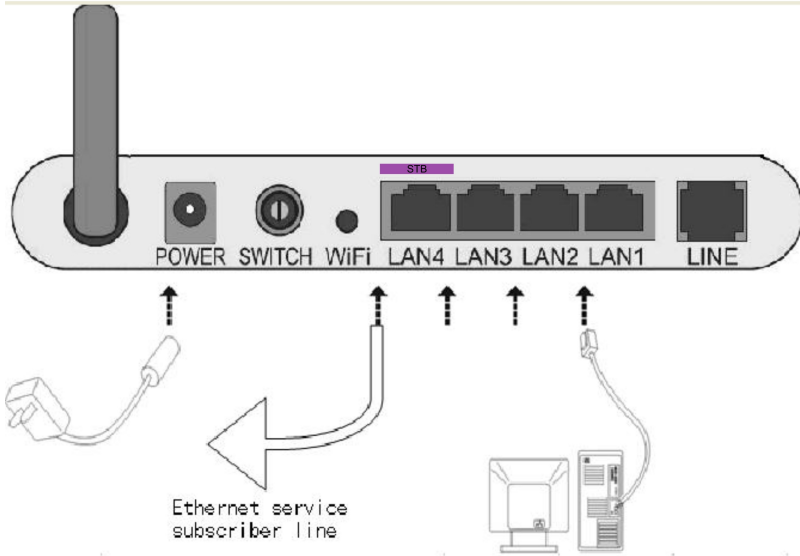
FIGURE 4 ETHERNET UPLINK CONNECTIONS
