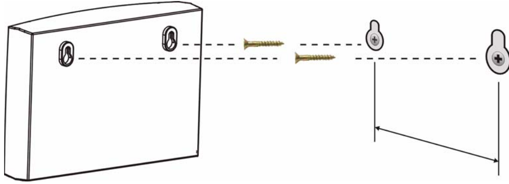
Figure 77 Wall-mounting Example
